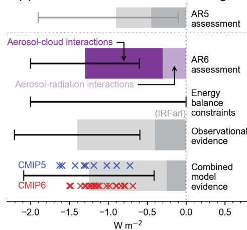
Figure TS.15 | Contribution to (a) effective radiative forcing (ERF) and (b) global surface temperature change from component emissions for 1750–2019 based on Coupled Model Intercomparison Project Phase 6 (CMIP6) models and (c) net aerosol ERF for 1750–2014 from different lines of evidence. The intent of this figure is to show advances since AR5 in the understanding of (a) emissions-based ERF, (b) global surface temperature response for short-lived climate forcers as estimated in Chapter 6, and (c) aerosol ERF from different lines of evidence as assessed in Chapter 7. In panel (a), ERFs for well-mixed greenhouse gases (WMGHGs) are from the analytical formulae. ERFs for other components are multi-model means based on Earth system model simulations that quantify the effect of individual components. The derived emissions-based ERFs are rescaled to match the concentration-based ERFs in Figure 7.6. Error bars are 5–95% and for the ERF account for uncertainty in radiative efficiencies and multi-model error in the means. In panel (b), the global mean temperature response is calculated from the ERF time series using an impulse response function. In panel (c), the AR6 assessment is based on energy balance constraints, observational evidence from satellite retrievals, and climate model-based evidence. For each line of evidence, the assessed best-estimate contributions from ERF due to aerosol–radiation interactions (ERF ari ) and aerosol–cloud interactions (ERF aci ) are shown with darker and paler shading, respectively. Estimates from individual CMIP Phase 5 (CMIP5) and CMIP6 models are depicted by blue and red crosses, respectively. The observational assessment for ERF ari is taken from the instantaneous forcing due to aerosol–radiation interactions (IRF ari ). Uncertainty ranges are given in black bars for the total aerosol ERF and depict very likely ranges. {6.4.2, Figure 6.12, 7.3.3, Cross-Chapter Box 7.1, Table 7.8, Figure 7.5}
