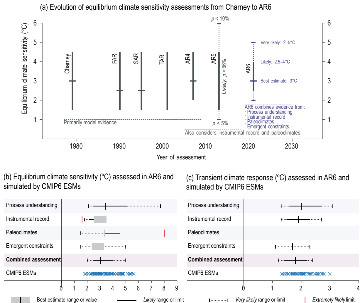
Figure TS.16 | (a) Evolution of equilibrium climate sensitivity (ECS) assessments from the Charney Report through a succession of IPCC Assessment Reports to AR6, and lines of evidence and combined assessment for (b) ECS and (c) transient climate response (TCR) in AR6. The intent of this figure is to show the progression in estimates of ECS, including uncertainty and the lines of evidence used for assessment, and to show the lines of assessment used to assess ECS and TCR in AR6. In panel (a), the lines of evidence considered are listed below each assessment. Best estimates are marked by horizontal bars, likely ranges by vertical bars, and very likely ranges by dotted vertical bars. In panel (b) and (c), assessed ranges are taken from Tables 7.13 and 7.14 for ECS and TCR respectively. Note that for the ECS assessment based on both the instrumental record and paleoclimates, limits (i.e., one-sided distributions) are given, which have twice the probability of being outside the maximum/minimum value at a given end, compared to ranges (i.e., two-tailed distributions) which are given for the other lines of evidence. For example, the extremely likely limit of greater than 95% probability corresponds to one side of the very likely (5% to 95%) range. Best estimates are given as either a single number or by a range represented by grey box. Coupled Model Intercomparison Project Phase 6 (CMIP6) Earth system model (ESM) values are not directly used as a line of evidence but are presented on the figure for comparison. {1.5, 7.5; Tables 7.13 and 7.14; Figure 7.18}
