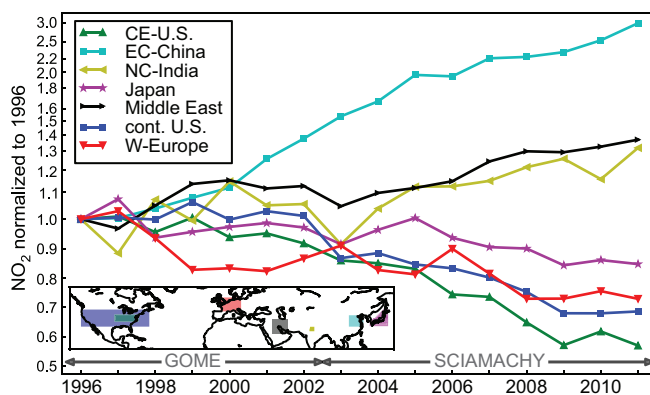
Figure 2.8 | Relative changes in tropospheric \text{NO}_2 column amounts (logarithmic scale) in seven selected world regions dominated by high \text{NO}_x emissions. Values are normalized for 1996 and derived from the GOME (Global Ozone Monitoring Experiment) instrument from 1996 to 2002 and SCIAMACHY (Scanning Imaging Spectrometer for Atmospheric Cartography) from 2003 to 2011 (Hilboll et al., 2013). The regions are indicated in the map inset.
