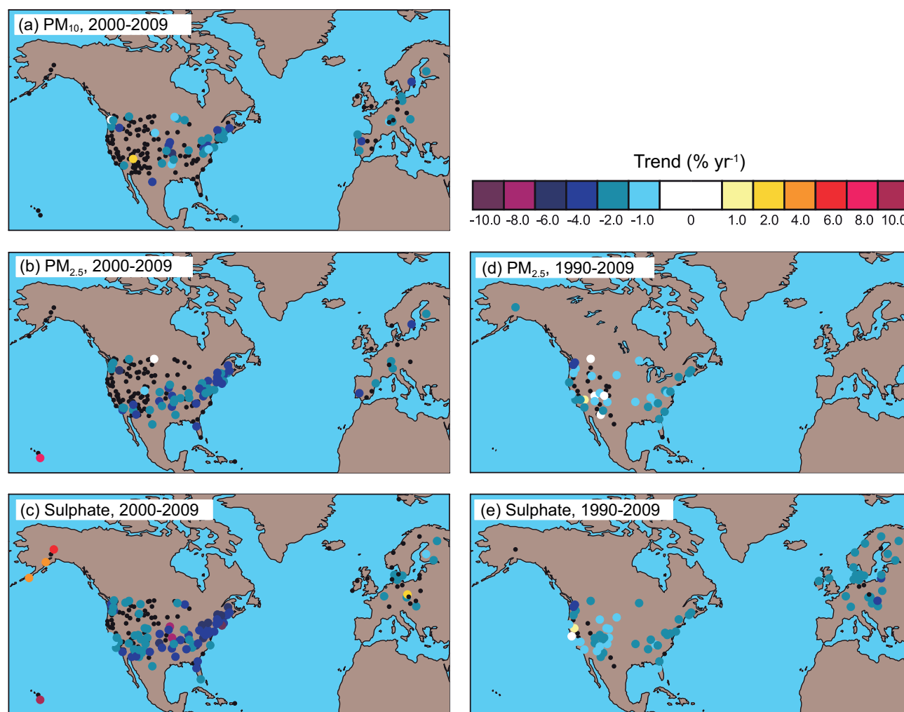
Figure 2.10 | Trends in particulate matter ( \text{PM}_{10} and \text{PM}_{2.5} with aerodynamic diameters <10 and <2.5 \mu\text{m} , respectively) and sulphate in Europe and USA for two overlapping periods 2000–2009 (a, b, c) and 1990–2009 (d, e). The trends are based on measurements from the EMEP (Torseth et al., 2012) and IMPROVE (Hand et al., 2011) networks in Europe and USA, respectively. Sites with significant trends (i.e., a trend of zero lies outside the 95% confidence interval) are shown in colour; black dots indicate sites with non-significant trends.
