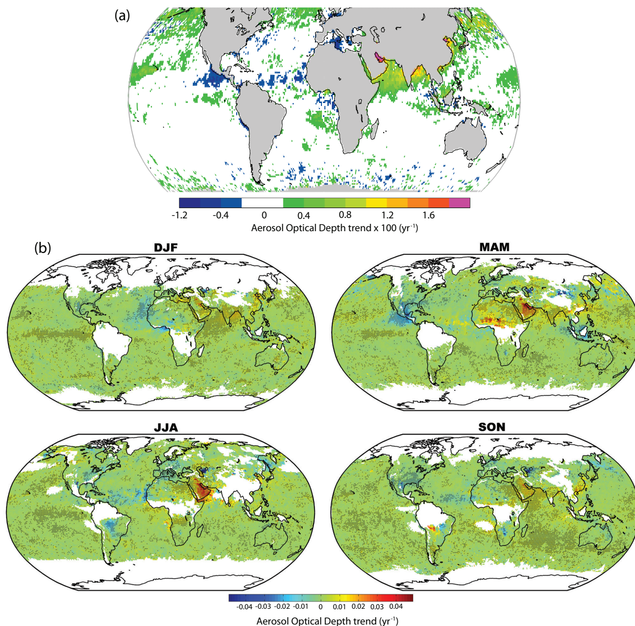
Figure 2.9 | (a) Annual average aerosol optical depth (AOD) trends at 0.55 \mu\text{m} for 2000–2009, based on de-seasonalized, conservatively cloud-screened MODIS aerosol data over oceans (Zhang and Reid, 2010). Negative AOD trends off Mexico are due to enhanced volcanic activity at the beginning of the record. Most non-zero trends are significant (i.e., a trend of zero lies outside the 95% confidence interval). (b) Seasonal average AOD trends at 0.55 \mu\text{m} for 1998–2010 using SeaWiFS data (Hsu et al., 2012). White areas indicate incomplete or missing data. Black dots indicate significant trends (i.e., a trend of zero lies outside the 95% confidence interval).
