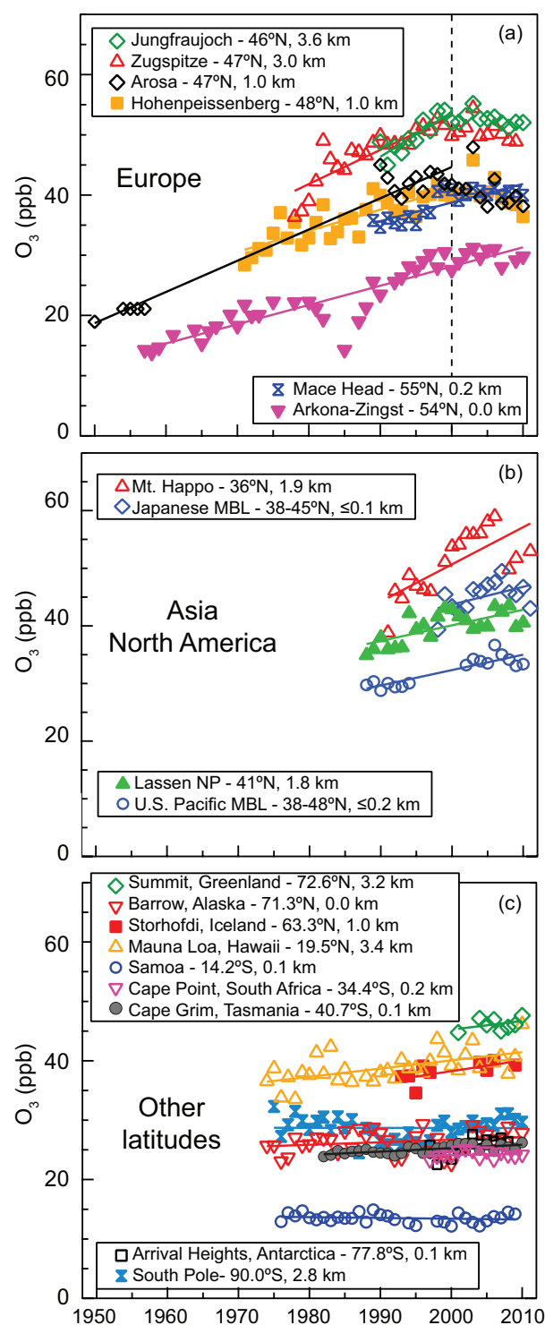
Figure 2.7 | Annual average surface ozone concentrations from regionally representative ozone monitoring sites around the world. (a) Europe. (b) Asia and North America. (c) Remote sites in the Northern and Southern Hemispheres. The station name in the legend is followed by its latitude and elevation. Time series include data from all times of day and trend lines are linear regressions following the method of Parrish et al. (2012). Trend lines are fit through the full time series at each location, except for Jungfraujoch, Zugspitze, Arosa and Hohenpeissenberg where the linear trends end in 2000 (indicated by the dashed vertical line in (a)). Twelve of these 19 sites have significant positive ozone trends (i.e., a trend of zero lies outside the 95% confidence interval); the seven sites with non-significant trends are: Japanese MBL (marine boundary layer), Summit (Greenland), Barrow (Alaska), Storhofdi (Iceland), Samoa (tropical South Pacific Ocean), Cape Point (South Africa) and South Pole (Antarctica).
