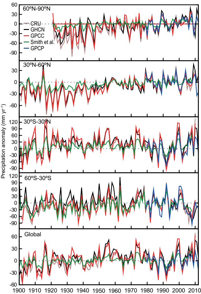
Figure 2.28 | Annual precipitation anomalies averaged over land areas for four latitudinal bands and the globe from five global precipitation data sets relative to a 1981–2000 climatology.
