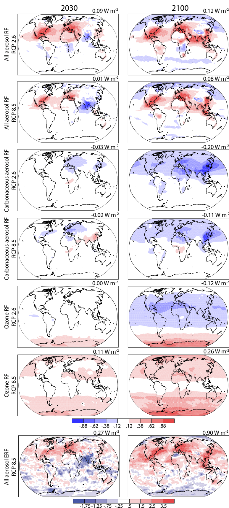
Figure 8.26 | Multi-model mean RF ( \text{W m}^{-2} ) due to aerosol–radiation interaction of all anthropogenic aerosols (first and second rows) and anthropogenic carbonaceous (BC+OC) aerosols (third and fourth rows), and total ozone (fifth and sixth rows) in 2030 (left) and 2100 (right) relative to 2000 for RCP2.6 (top each) and RCP8.5 (bottom each) based on the ACCMIP simulations. The seventh row shows multi-model mean ERF ( \text{W m}^{-2} ) by all anthropogenic aerosols in 2030 (left) and 2100 (right) relative to 2000 for RCP8.5. Global area-weighted means are given in the upper right of each panel.
