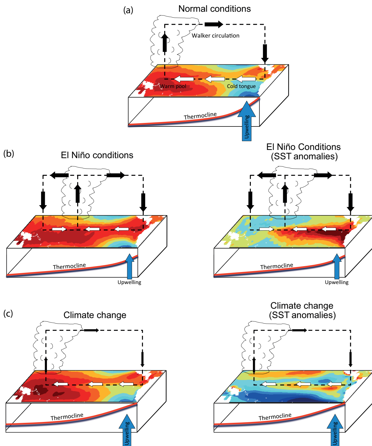
Figure 14.12 | Idealized schematic showing atmospheric and oceanic conditions of the tropical Pacific region and their interactions during normal conditions, El Niño conditions, and in a warmer world. (a) Mean climate conditions in the tropical Pacific, indicating sea surface temperatures (SSTs), surface wind stress and associated Walker Circulation, the mean position of convection and the mean upwelling and position of the thermocline. (b) Typical conditions during an El Niño event. SSTs are anomalously warm in the east; convection moves into the central Pacific; the trade winds weaken in the east and the Walker Circulation is disrupted; the thermocline flattens and the upwelling is reduced. (c) The likely mean conditions under climate change derived from observations, theory and coupled General Circulation Models (GCMs). The trade winds weaken; the thermocline flattens and shoals; the upwelling is reduced although the mean vertical temperature gradient is increased; and SSTs (shown as anomalies with respect to the mean tropical-wide warming) increase more on the equator than off. Diagrams with absolute SST fields are shown on the left, diagrams with SST anomalies are shown on the right. For the climate change fields, anomalies are expressed with respect to the basin average temperature change so that blue colours indicate a warming smaller than the basin mean, not a cooling (Collins et al., 2010).
