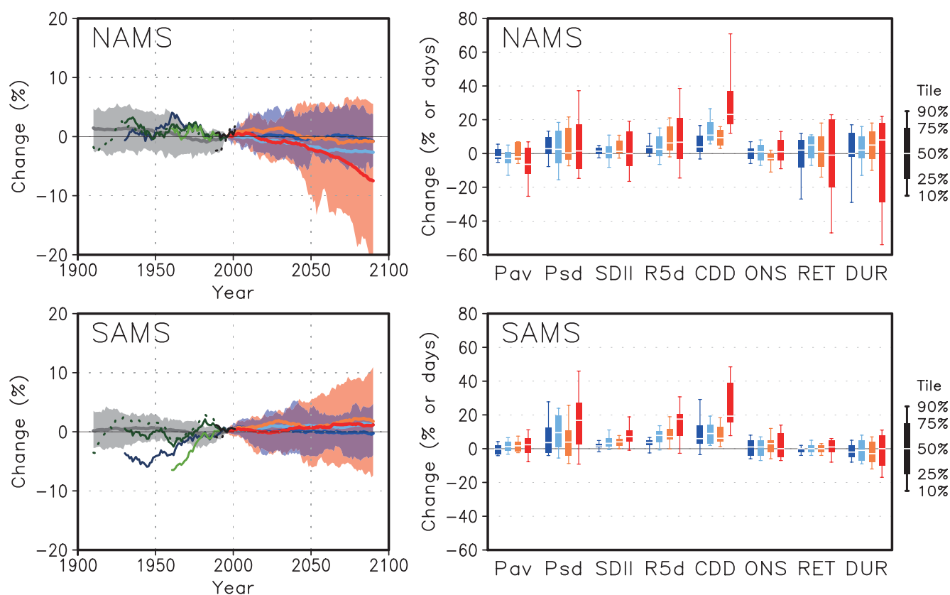
Figure 14.6 | As in Figure 14.4, except for (upper) North America Monsoon System (NAMS) and (lower) South America Monsoon System (SAMS).
