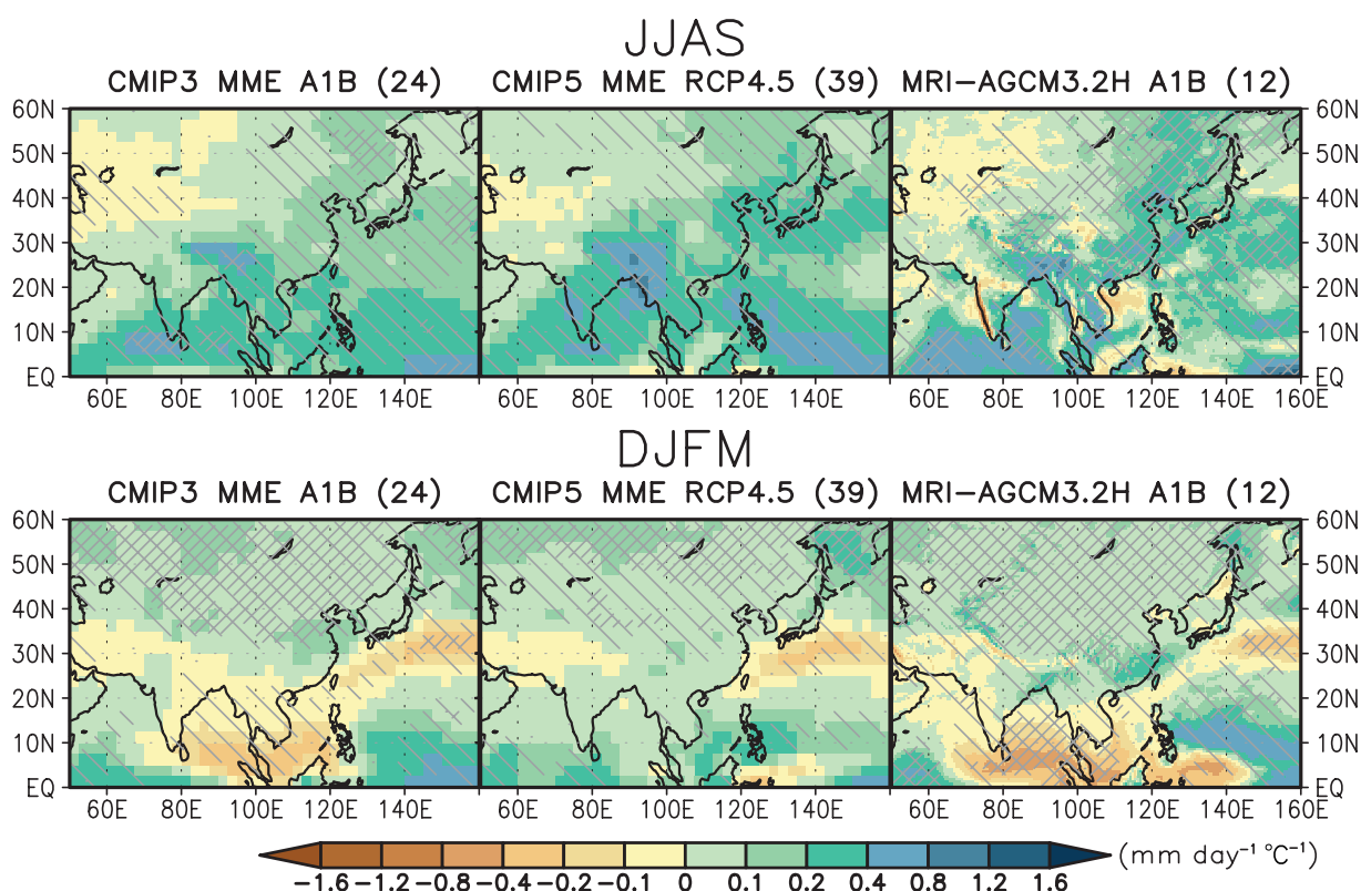
Figure 14.24 | Maps of precipitation changes for Central, North, East and South Asia in 2080–2099 with respect to 1986–2005 in June to September (above) and December to March (below) in the SRES A1B scenario with 24 CMIP3 models (left), and in the RCP4.5 scenario with 39 CMIP5 models (middle). Right figures are the precipitation changes in 2075–2099 with respect to 1979–2003 in the SRES A1B scenario with the 12-member 60-km mesh Meteorological Research Institute (MRI)-Atmospheric General Circulation Model 3.2 (AGCM3.2) multi-physics, multi-sea surface temperature (SST) ensembles (Endo et al., 2012). Precipitation changes are normalized by the global annual mean surface air temperature changes in each scenario. Light hatching denotes where more than 66% of models (or members) have the same sign with the ensemble mean changes, while dense hatching denotes where more than 90% of models (or members) have the same sign with the ensemble mean changes.
