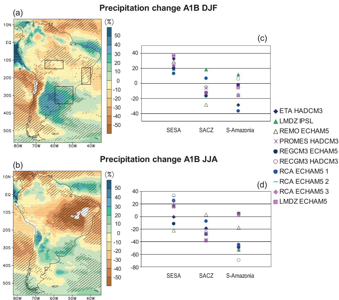
Figure 14.21 | (a) December, January and February (DJF) and (b) June, July and August (JJA) relative precipitation change in 2071–2100 with respect to 1961–1990 in the A1B scenario from an ensemble of 10 Regional Climate Models (RCMs) participating in the Europe–South America Network for Climate Change Assessment and Impact Studies-La Plata Basin (CLARIS-LPB) Project. Hatching denotes areas where 8 out of 10 RCMs agree in the sign of the relative change. (c) DJF and (d) JJA dispersion among regional model projections of precipitation changes averaged over land grid points in Southeastern South America (SESA, 35°S to 25°S, 60°W to 50°W), South Atlantic Convergence Zone (SACZ, 25°S to 15°S, 45°W to 40°W) and southern Amazonia (15°S to 10°S, 65°W to 55°W), indicated by the boxes in (a).
