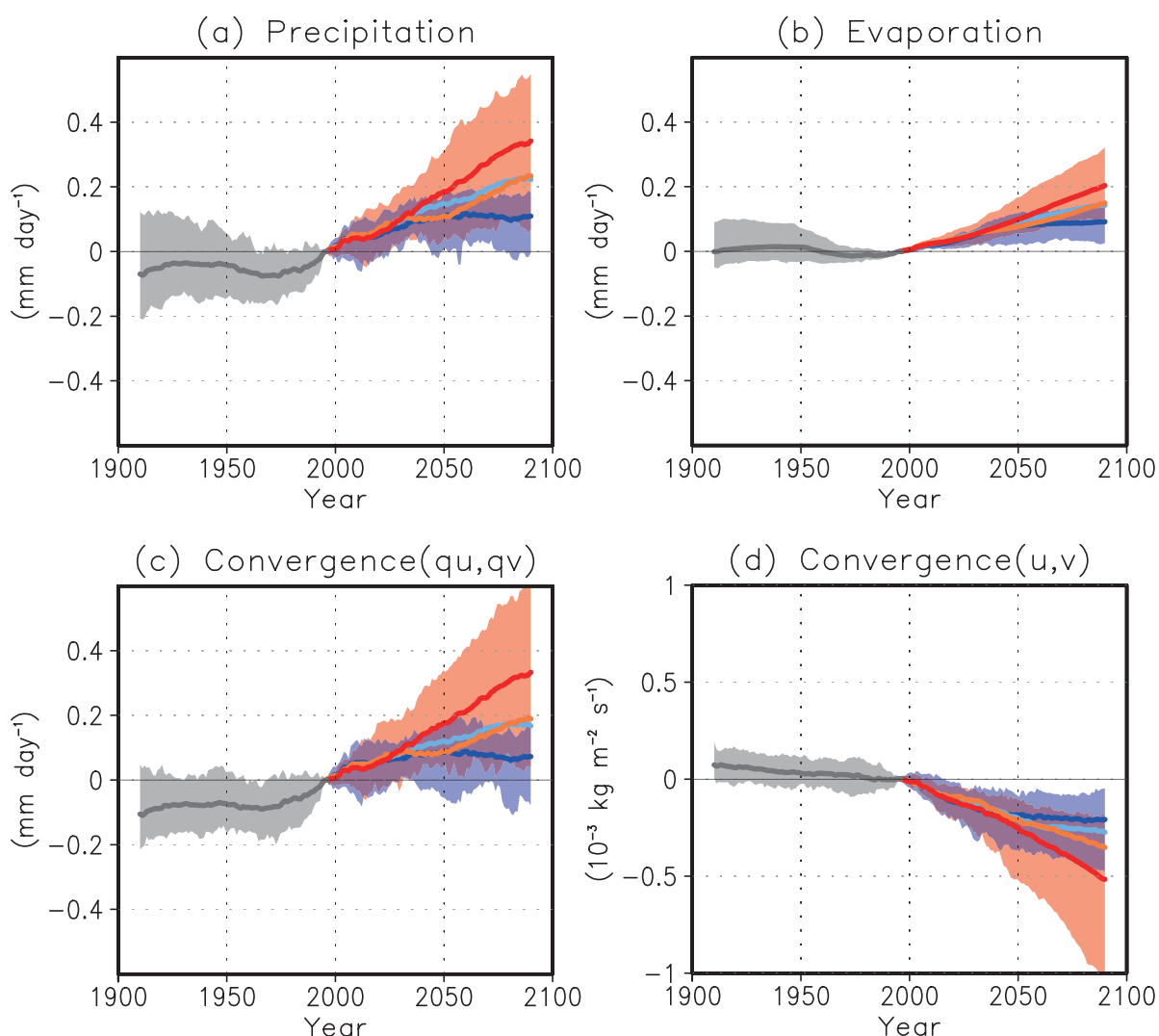
Figure 14.2 | Time series of simulated anomalies, smoothed with a 20-year running mean over the global land monsoon domain for (a) precipitation (mm day -1 ), (b) evaporation (mm day -1 ), (c) water vapour flux convergence in the lower (below 500 hPa) troposphere (mm day -1 ), and (d) wind convergence in the lower troposphere (10 -3 kg m -2 s -1 ), relative to the present-day (1986–2005), based on CMIP5 multi-model monthly outputs. Historical (grey; 29 models), RCP2.6 (dark blue; 20 models), RCP4.5 (light blue; 24 models), RCP6.0 (orange; 16 models), and RCP8.5 (red; 24 models) simulations are shown in the 10th and 90th percentile (shading), and in all model averages (thick lines).
