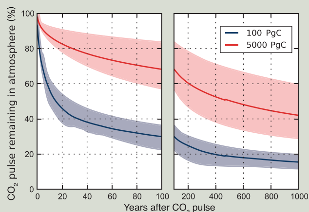
TFE.7, Figure 1 | Percentage of initial atmospheric \text{CO}_2 perturbation remaining in the atmosphere in response to an idealized instantaneous \text{CO}_2 emission pulse in year 0 as calculated by a range of coupled climate–carbon cycle models. Multi-model mean (line) and the uncertainty interval (maximum model range, shading) simulated during 100 years (left) and 1 kyr (right) following the instantaneous emission pulse of 100 PgC (blue) and 5,000 PgC (red). {Box 6.1, Figure 1}
