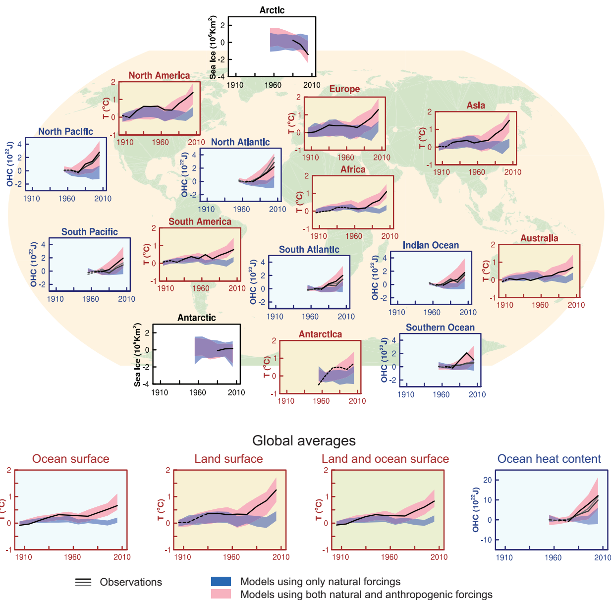
Figure TS.12 | Comparison of observed and simulated change in the climate system, at regional scales (top panels) and global scales (bottom four panels). Brown panels are land surface temperature time series, blue panels are ocean heat content time series and white panels are sea ice time series (decadal averages). Each panel shows observations (black or black and shades of grey), and the 5 to 95% range of the simulated response to natural forcings (blue shading) and natural and anthropogenic forcings (pink shading), together with the corresponding ensemble means (dark blue and dark red respectively). The observed surface temperature is from the Hadley Centre/Climatic Research Unit gridded surface temperature data set 4 (HadCRUT4). Three observed records of ocean heat content (OHC) are shown. Sea ice anomalies (rather than absolute values) are plotted and based on models in Figure 10.16. The observations lines are either solid or dashed and indicate the quality of the observations and estimates. For land and ocean surface temperatures panels and precipitation panels, solid observation lines indicate where spatial coverage of areas being examined is above 50% coverage and dashed observation lines where coverage is below 50%. For example, data coverage of Antarctica never goes above 50% of the land area of the continent. For ocean heat content and sea ice panels the solid observations line is where the coverage of data is good and higher in quality, and the dashed line is where the data coverage is only adequate. This figure is based on Figure 10.21 except presented as decadal averages rather than yearly averages. Further detail regarding the related Figure SPM.6 is given in the TS Supplementary Material. {Figure 10.21}
