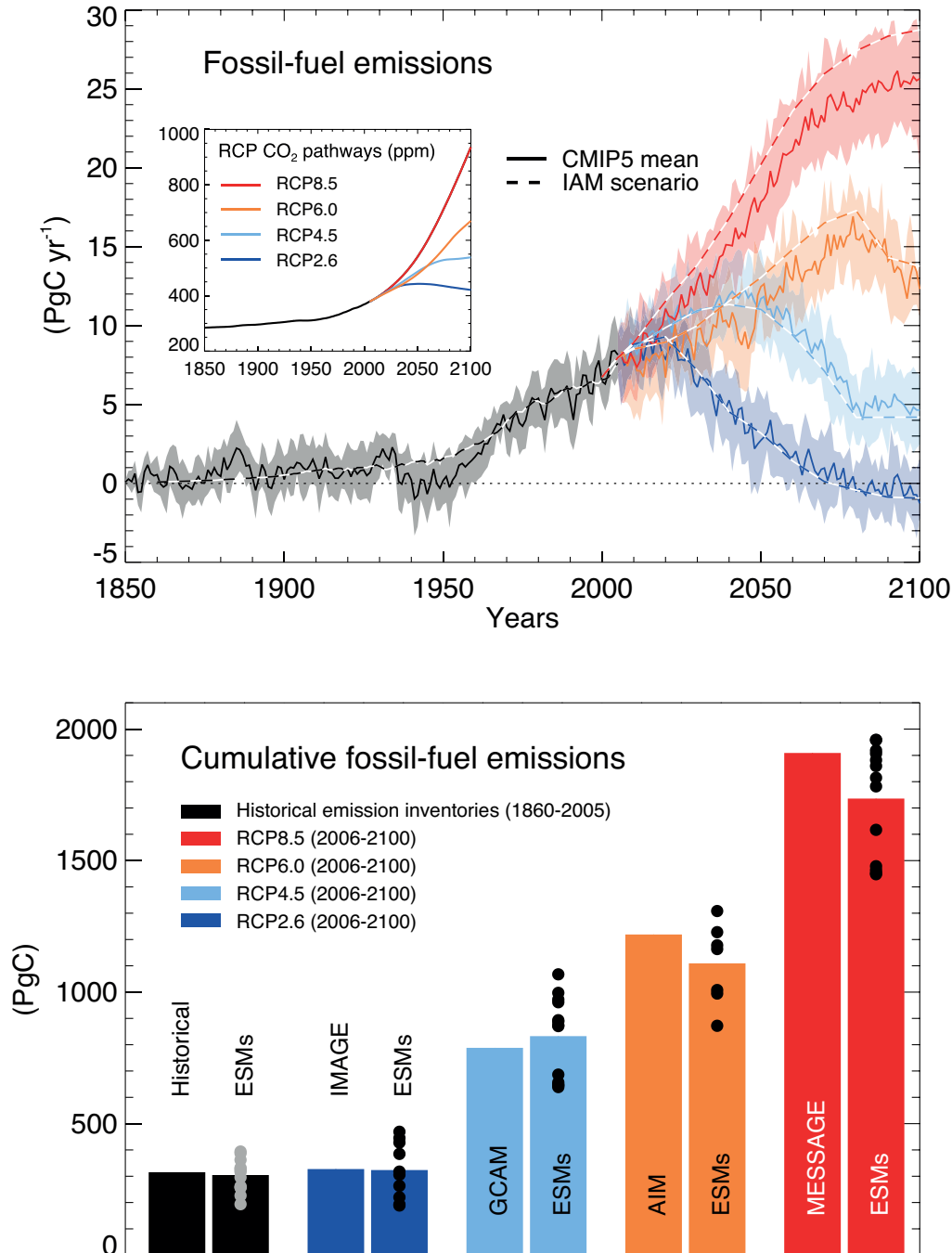
Figure TS.19 | Compatible fossil fuel emissions simulated by the CMIP5 models for the four RCP scenarios. (Top) Time series of annual emission (PgC yr -1 ). Dashed lines represent the historical estimates and RCP emissions calculated by the Integrated Assessment Models (IAMs) used to define the RCP scenarios, solid lines and plumes show results from CMIP5 Earth System Models (ESMs, model mean, with one standard deviation shaded). (Bottom) Cumulative emissions for the historical period (1860–2005) and 21st century (defined in CMIP5 as 2006–2100) for historical estimates and RCP scenarios. Left bars are cumulative emissions from the IAMs, right bars are the CMIP5 ESMs multi-model mean estimate and dots denote individual ESM results. From the CMIP5 ESMs results, total carbon in the land-atmosphere–ocean system can be tracked and changes in this total must equal fossil fuel emissions to the system. Hence the compatible emissions are given by cumulative emissions = \Delta C_A + \Delta C_L + \Delta C_O , while emission rate = d/dt [C_A + C_L + C_O] , where C_A , C_L , C_O are carbon stored in atmosphere, land and ocean respectively. Other sources and sinks of CO 2 such as from volcanism, sedimentation or rock weathering, which are very small on centennial time scales are not considered here. [Box 6.4; Figure 6.25]
