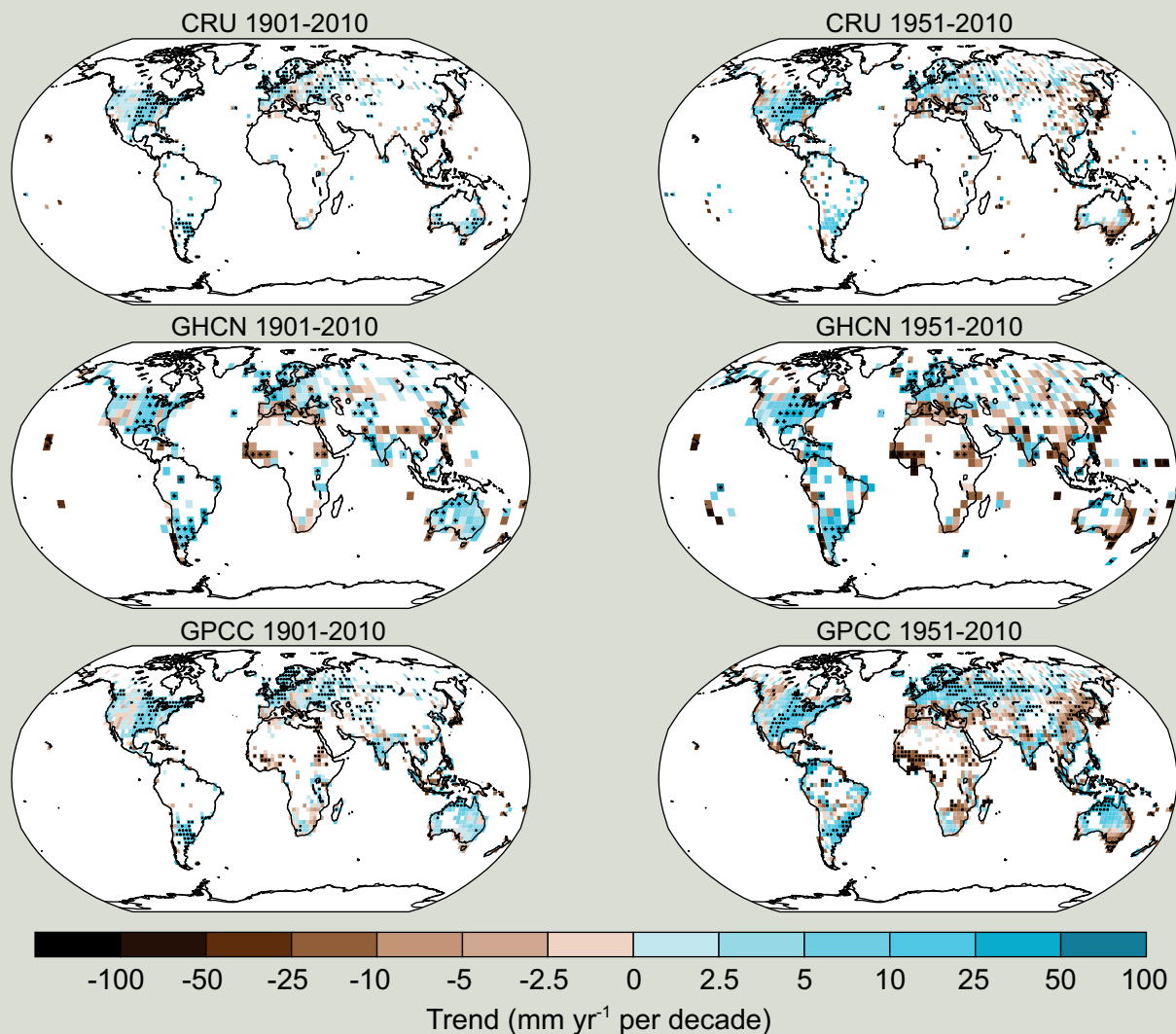
TFE.1, Figure 2 | Maps of observed precipitation change over land from 1901 to 2010 (left-hand panels) and 1951 to 2010 (right-hand panels) from the Climatic Research Unit (CRU), Global Historical Climatology Network (GHCN) and Global Precipitation Climatology Centre (GPCC) data sets. Trends in annual accumulation have been calculated only for those grid boxes with greater than 70% complete records and more than 20% data availability in first and last decile of the period. White areas indicate incomplete or missing data. Black plus signs (+) indicate grid boxes where trends are significant (i.e., a trend of zero lies outside the 90% confidence interval). Further detail regarding the related Figure SPM.2 is given in the TS Supplementary Material. {Figure 2.29; 2.5.1}
