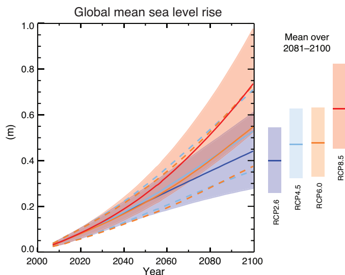
Figure TS.22 | Projections from process-based models of global mean sea level (GMSL) rise relative to 1986–2005 for the four RCP scenarios. The solid lines show the median projections, the dashed lines show the likely ranges for RCP4.5 and RCP6.0, and the shading the likely ranges for RCP2.6 and RCP8.5. The time means for 2081–2100 are shown as coloured vertical bars. See Sections 13.5.1 and 13.5.3 and Supplementary Material for methods. Based on current understanding, only the collapse of the marine-based sectors of the Antarctic ice sheet, if initiated, could cause GMSL to rise substantially above the likely range during the 21st century. This potential additional contribution cannot be precisely quantified but there is medium confidence that it would not exceed several tenths of a metre during the 21st century. Further detail regarding the related Figure SPM.9 is given in the TS Supplementary Material. {Table 13.5; Figures 13.10, 13.11}
