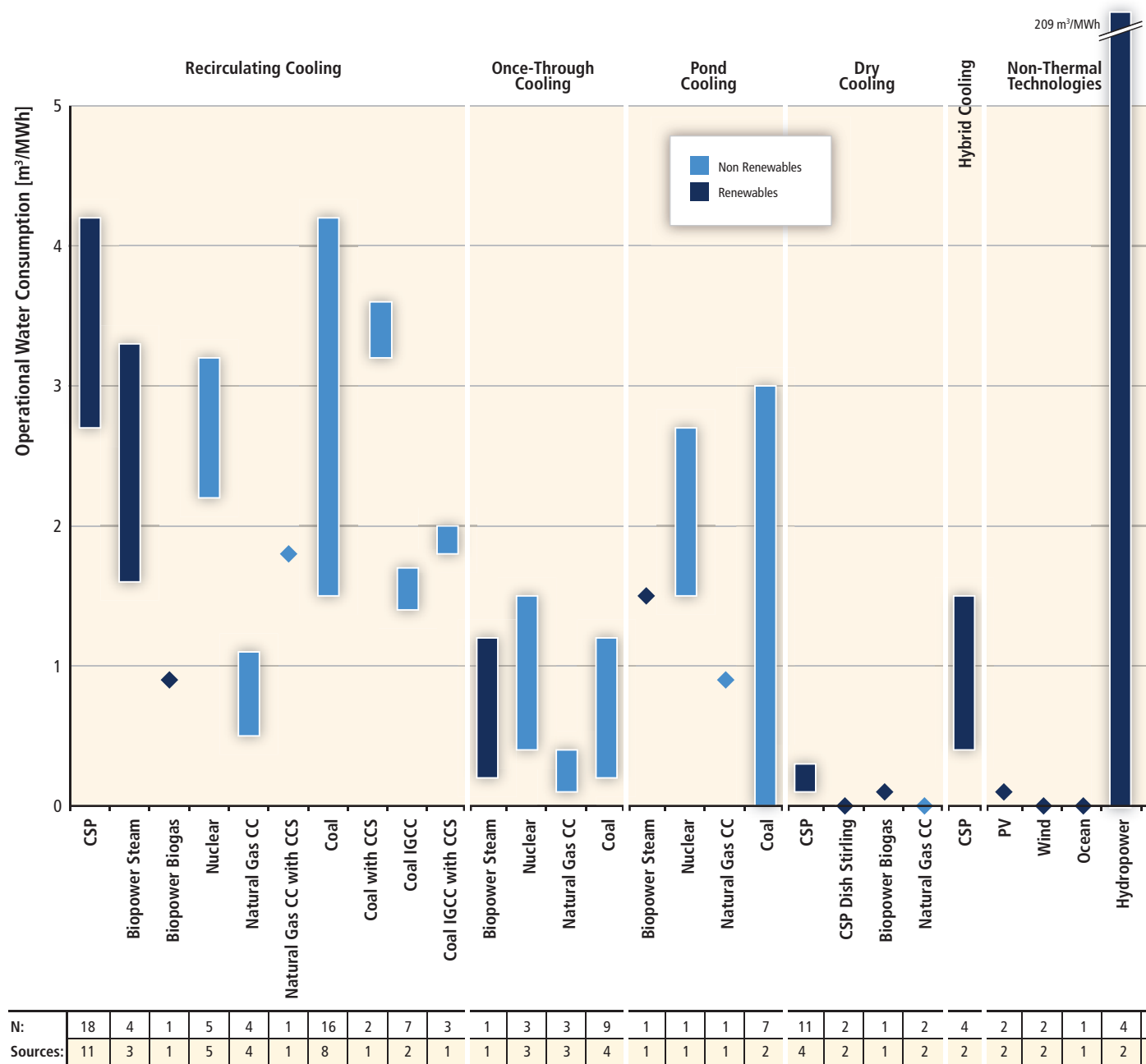
Figure TS.9.5 | Ranges of rates of operational water consumption by thermal and non-thermal electricity-generating technologies based on a review of available literature (m³/MWh). Bars represent absolute ranges from available literature, diamonds single estimates; n represents the number of estimates reported in the sources. Methods and references used in this literature review are reported in Annex II. Note that upper values for hydropower result from a few studies measuring gross evaporation values, and may not be representative (see Box 5.2). [Figure 9.14]
