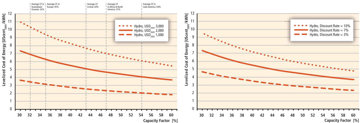
Figure TS.5.3 | Recent and near-term estimated levelized cost of hydropower (a) as a function of capacity factor and investment cost * , ** , *** ; and (b) as a function of capacity factor and discount rate ** , *** . [Figure 5.20]
