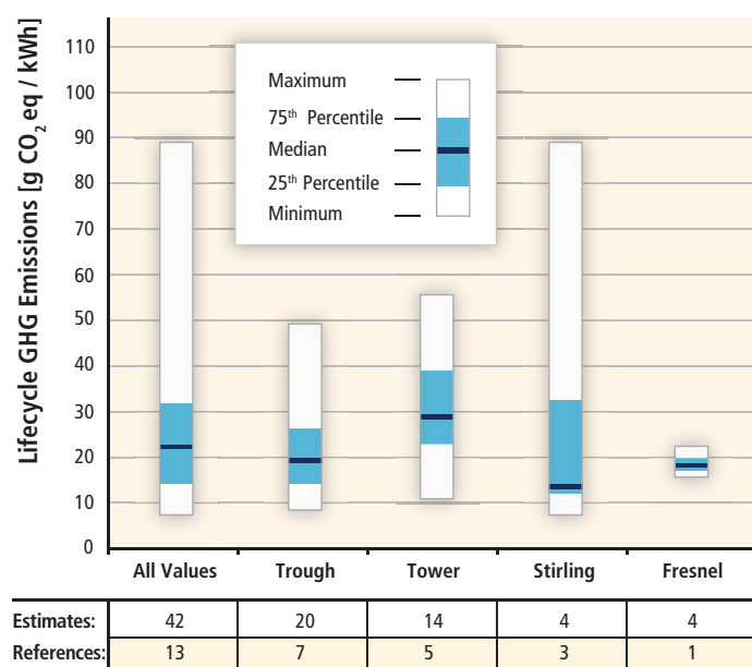
Figure TS.3.4 | GHG emissions from the life cycles of (top) PV modules and (bottom) CSP technologies. See Annex II for details of literature search and citations of literature contributing to the estimates displayed. [Figures 3.14, 3.15]
