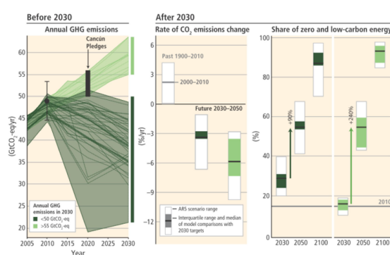
Figure SPM.12 | The implications of different 2030 greenhouse gas (GHG) emissions levels for the rate of carbon dioxide (CO 2 ) emissions reductions and low-carbon energy upscaling in mitigation scenarios that are at least as likely as not to keep warming throughout the 21st century below 2°C relative to pre-industrial levels (2100 CO 2 -equivalent concentrations of 430 to 530 ppm). The scenarios are grouped according to different emissions levels by 2030 (coloured in different shades of green). The left panel shows the pathways of GHG emissions (gigatonne of CO 2 -equivalent per year, GtCO 2 -eq/yr) leading to these 2030 levels. The black dot with whiskers gives historic GHG emission levels and associated uncertainties in 2010 as reported in Figure SPM.2. The black bar shows the estimated uncertainty range of GHG emissions implied by the Cancun Pledges. The middle panel denotes the average annual CO 2 emissions reduction rates for the period 2030–2050. It compares the median and interquartile range across scenarios from recent inter-model comparisons with explicit 2030 interim goals to the range of scenarios in the Scenario Database for WGIII AR5. Annual rates of historical emissions change (sustained over a period of 20 years) and the average annual CO 2 emission change between 2000 and 2010 are shown as well. The arrows in the right panel show the magnitude of zero and low-carbon energy supply upscaling from 2030 to 2050 subject to different 2030 GHG emissions levels. Zero- and low-carbon energy supply includes renewables, nuclear energy and fossil energy with carbon dioxide capture and storage (CCS) or bioenergy with CCS (BECCS). [Note: Only scenarios that apply the full, unconstrained mitigation technology portfolio of the underlying models (default technology assumption) are shown. Scenarios with large net negative global emissions (>20 GtCO 2 -eq/yr), scenarios with exogenous carbon price assumptions and scenarios with 2010 emissions significantly outside the historical range are excluded.] (Figure 3.3)
