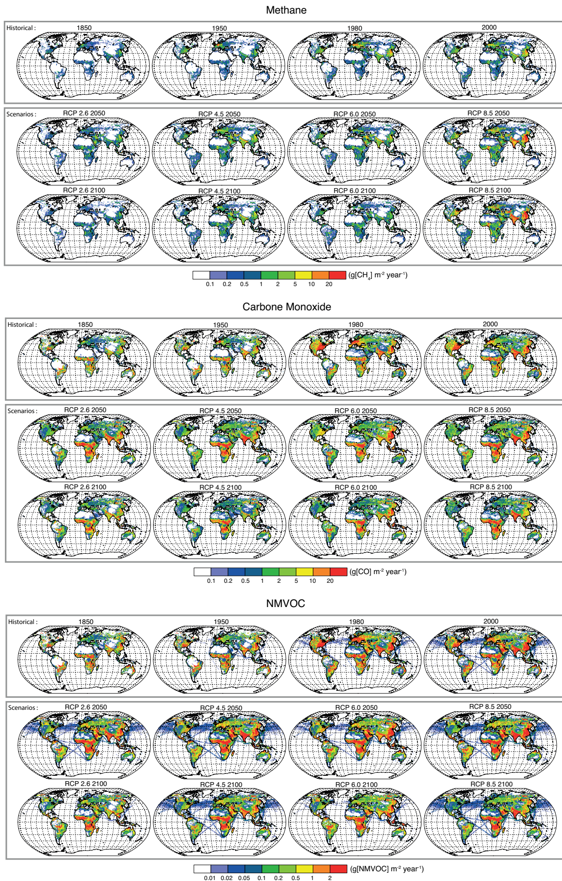
Figure 8.SM.2 | Time evolution of anthropogenic and biomass burning emissions 1850–2100 used in CMIP5/ACCIP following each RCP. Historical (1850–2000) values are from Lamarque et al. (2010). RCP values are from van Vuuren et al. (2011).
