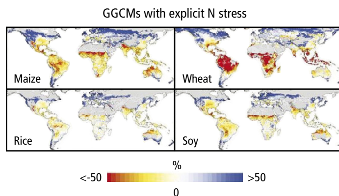
Figure 5.4 | AgMIP median yield changes (%) for RCP8.5 (2070–2099 in comparison to 1980–2010 baseline) with CO 2 effects and explicit nitrogen stress over five GGCMs x four Global Gridded Crop Models (GGCMs) for rainfed maize, wheat, rice, and soy (20 ensemble members from EPIC, GEPIC, pDSSAT, and PEGASUS; except for rice which has 15). Grey areas indicate historical areas with little to no yield capacity. All models use a 0.5°C grid, but there are differences in grid cells simulated to represent agricultural land. While some models simulated all land areas, others simulated only potential suitable cropland area according to evolving climatic conditions. Others utilised historical harvested areas in 2000 according to various data sources (Rosenzweig et al. 2014).
