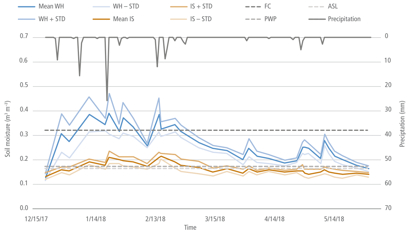
Figure 3.18 | Illustration of enhanced soil water retention in the Mechanized Micro Rainwater Harvesting compared to untreated Badia rangelands in Jordan, showing precipitation (PCP), sustained stress level resulting in decreased production, field capacity and wilting point for available soil moisture, and then measured soil moisture content between the two treatments (degraded rangeland and the restored rangeland with the Vallerani plough).
