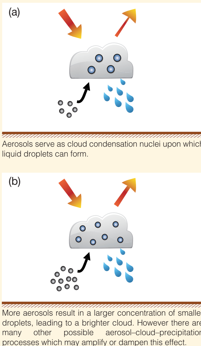
FAQ 7.2, Figure 2 | Overview of aerosol–cloud interactions and their impact on climate. Panels (a) and (b) represent a clean and a polluted low-level cloud, respectively.
