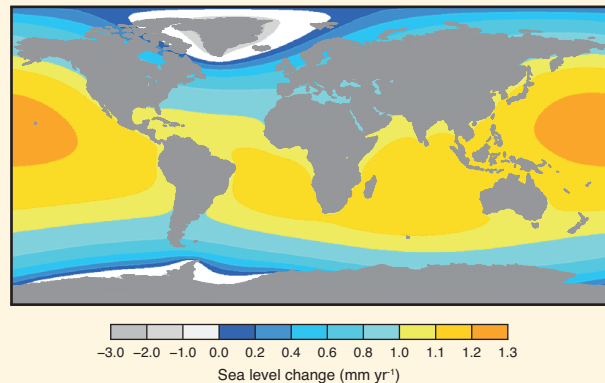
FAQ13.1, Figure 2 | Model output showing relative sea level change due to melting of the Greenland ice sheet and the West Antarctic ice sheet at rates of 0.5 mm yr -1 each (giving a global mean value for sea level rise of 1 mm yr -1 ). The modelled sea level changes are less than the global mean value in areas near the melting ice but enhanced further afield. (Adapted from Milne et al., 2009)
