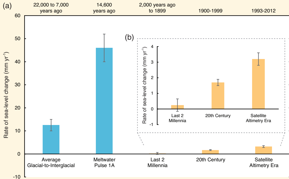
FAQ 5.2, Figure 1 | (a) Estimates of the average rate of global mean sea level change (in \text{mm yr}^{-1} ) for five selected time intervals: last glacial-to-interglacial transition; Meltwater Pulse 1A; last 2 millennia; 20th century; satellite altimetry era (1993–2012). Blue columns denote time intervals of transition from a glacial to an interglacial period, whereas orange columns denote the current interglacial period. Black bars indicate the range of likely values of the average rate of global mean sea level change. Note the overall higher rates of global mean sea level change characteristic of times of transition between glacial and interglacial periods. (b) Expanded view of the rate of global mean sea level change during three time intervals of the present interglacial.
